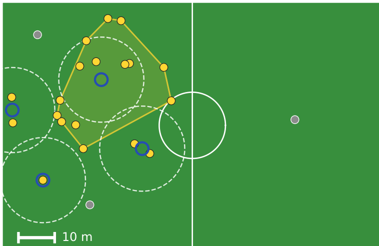
(c) Tactical clustering ( \delta = 11.75 m)
