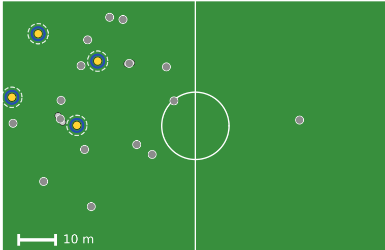
(a) Individual clustering ( \delta = 2.75 m)
