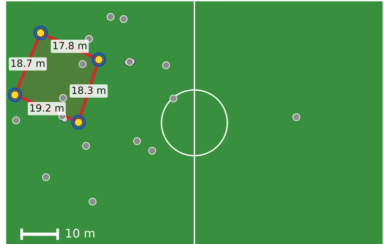
(b) Individual H_1 ( \delta = 2.75 m)
